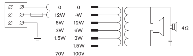
LC1-UM12E8 Circuit diagram
