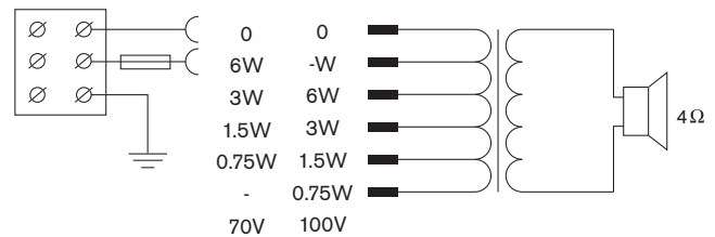
LC1-UM06E8 Circuit diagram
