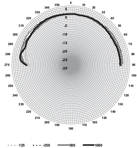
LC1-UM24E8 Frequency response
