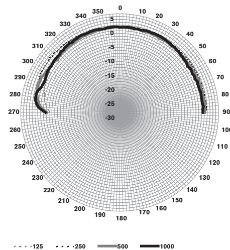
LC1-UM12E8 Frequency response
