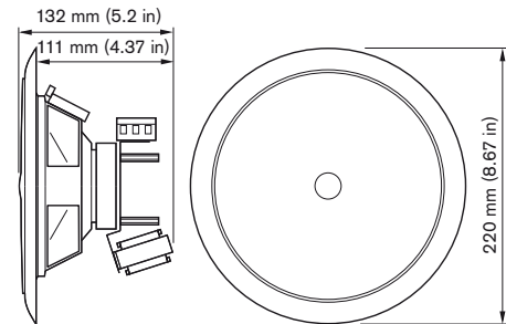
LC1-UM12E8 Dimensions in mm (in)
