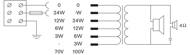
LC1-UM24E8 Circuit diagram
