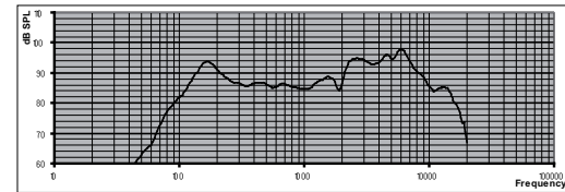
Frequency response LC3-UC06E
