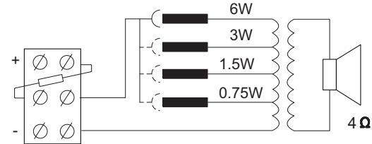
Circuit diagram LC3-UC06E
