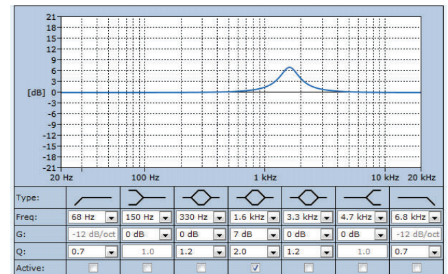
LC3-UC06E specified active equalization required for EN 54-24
